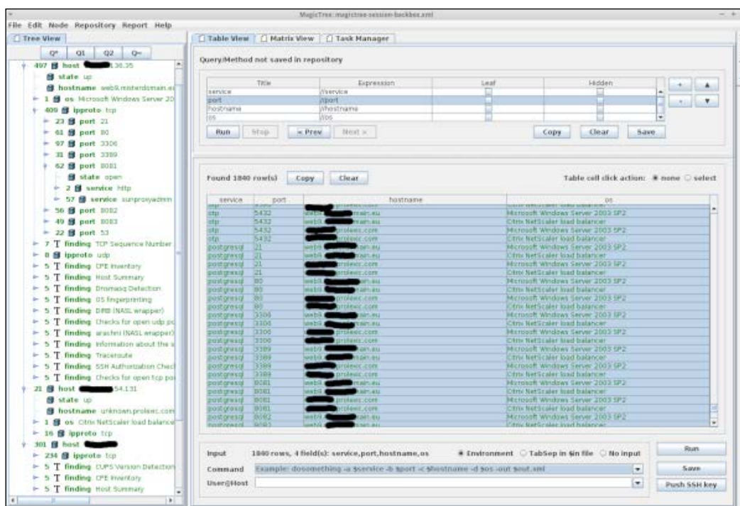
Custom query with relative ports, hostnames, and OSs
