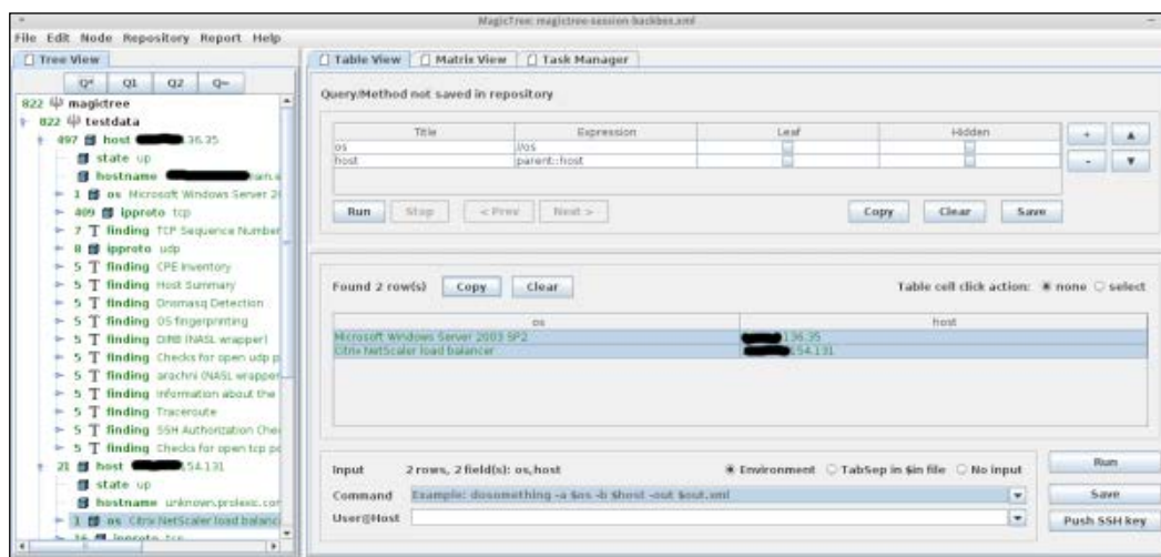
Running a query to view OSs
